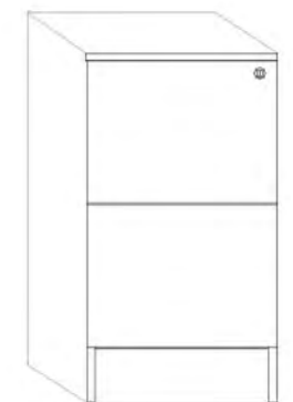
PS031 Side Pull W395x D580 x H725
