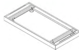
PS020 Standing Base W900 x D440 x H60
