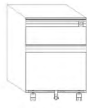
PS024 S Tyle Front Pull W395x D528 x H538
